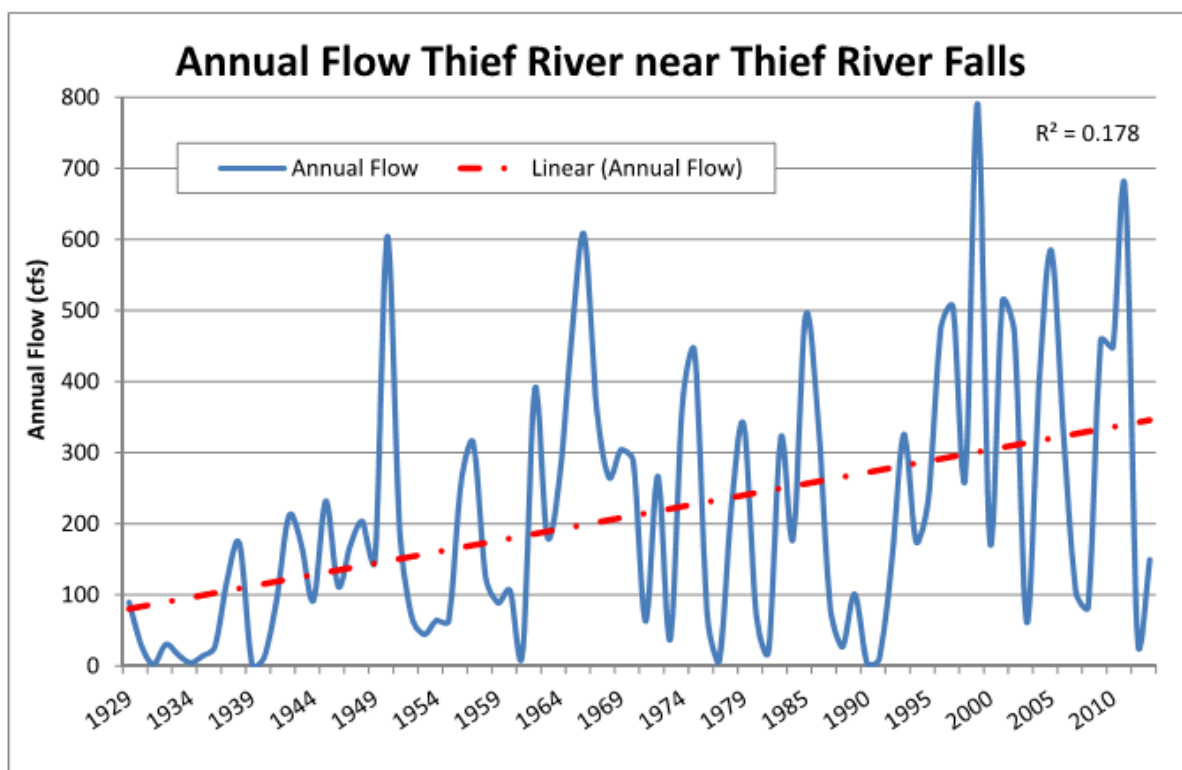
Figure 18: Annual Mean Flow at USGS Stream Gage 0507600 near Thief River Falls
