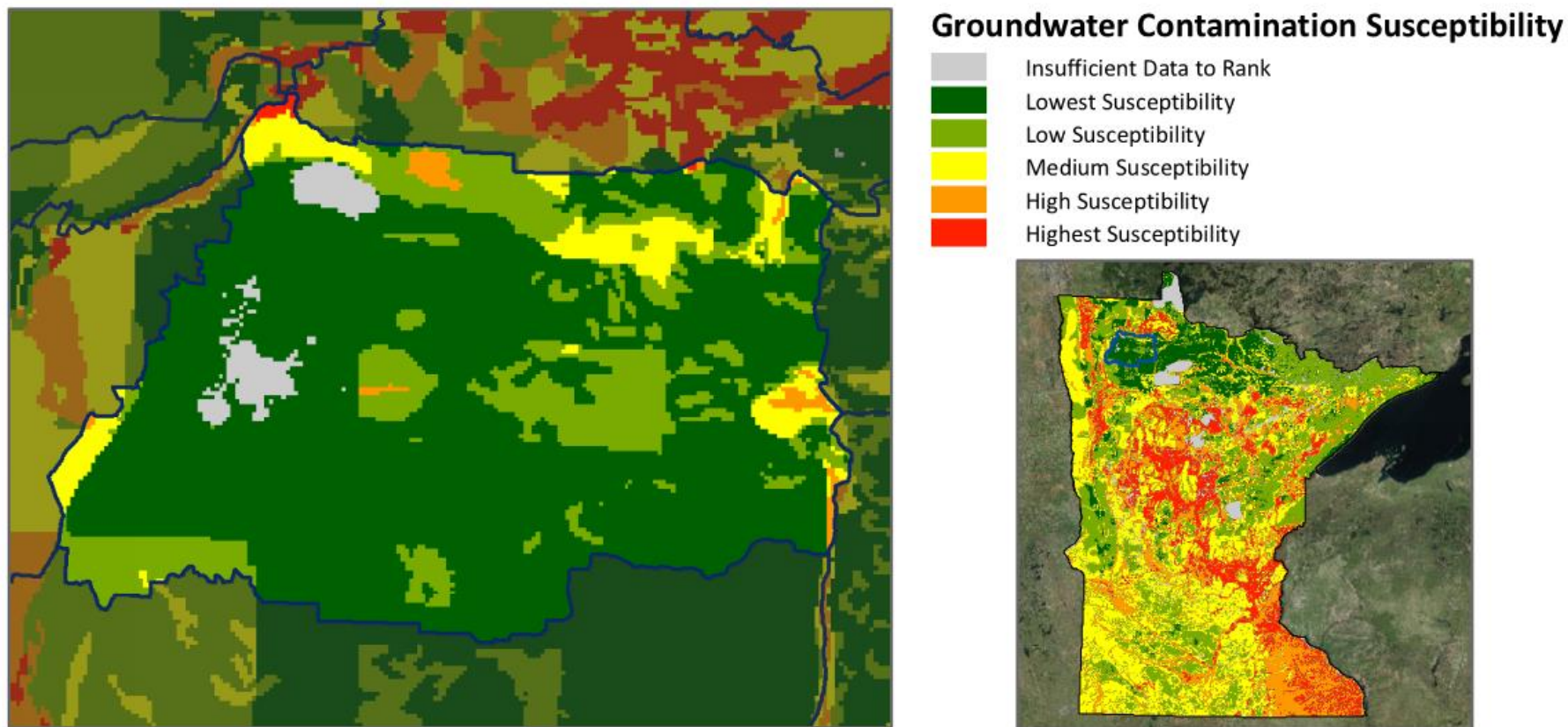
Figure 31: Groundwater Susceptibility for the Thief River Watershed.
