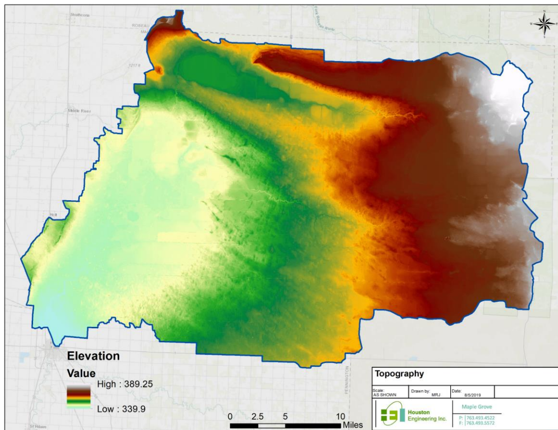
Figure 2: Thief River Watershed Topography
